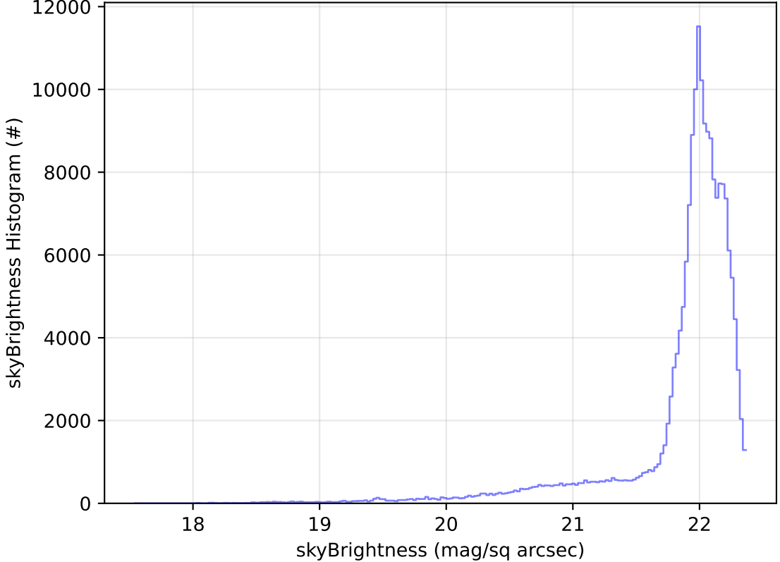
ddf_acor_sf10_lsf20_lsr10_v3.4_10yrs WFD g band: skyBrightness Histogram
