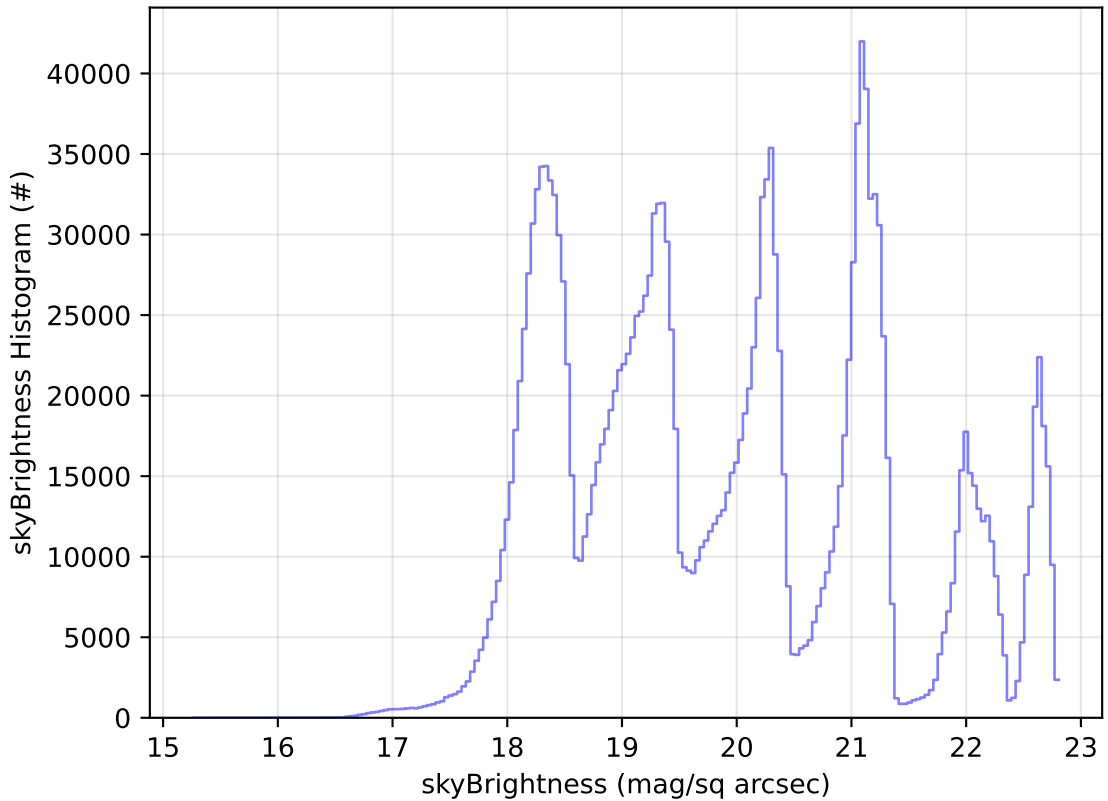
ddf_acor_sf10_lsf20_lsr10_v3.4_10yrs WFD all bands: skyBrightness Histogram
