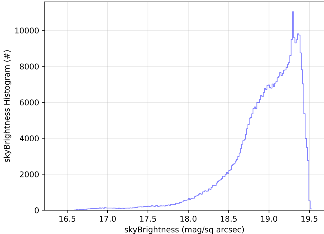
ddf_acor_sf10_lsf20_lsr10_v3.4_10yrs All sky z band: skyBrightness Histogram
