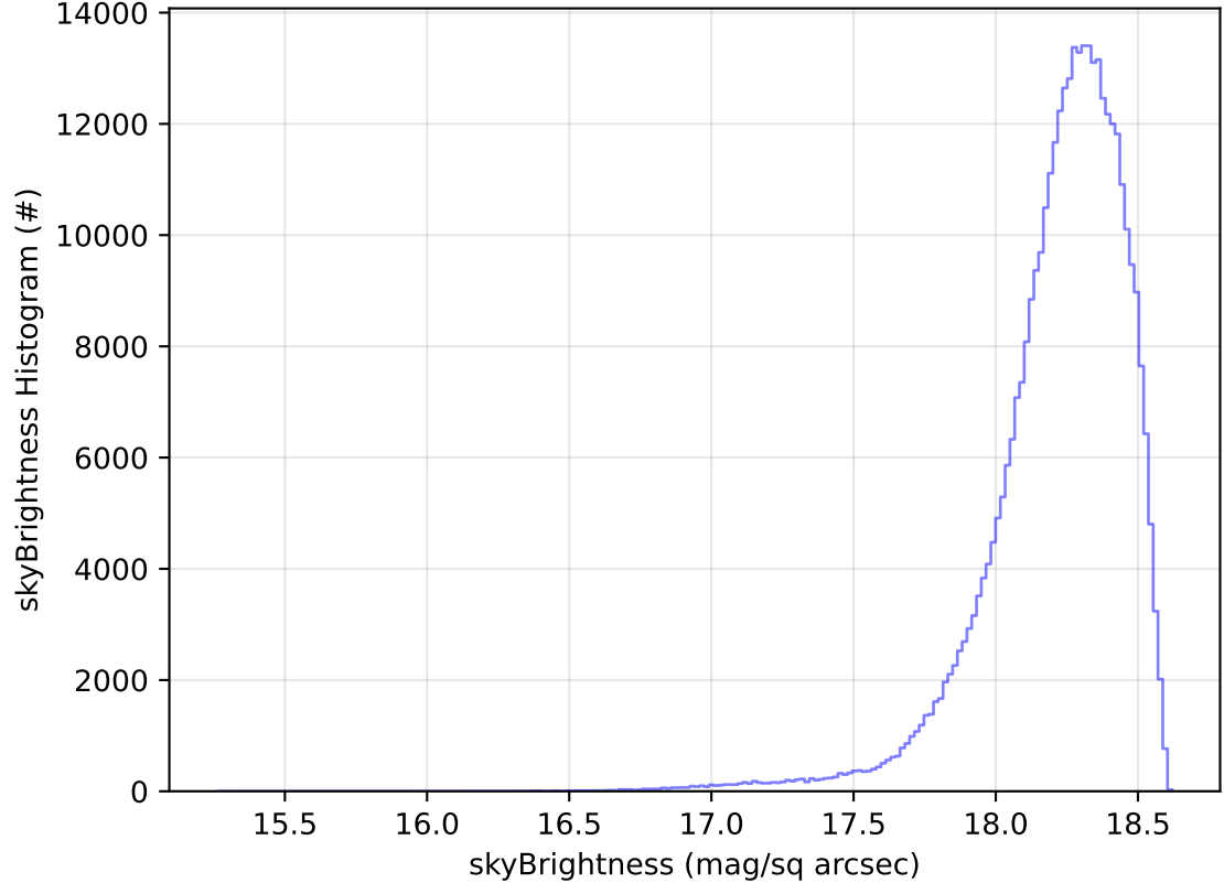
ddf_acor_sf10_lsf20_lsr10_v3.4_10yrs All sky y band: skyBrightness Histogram
