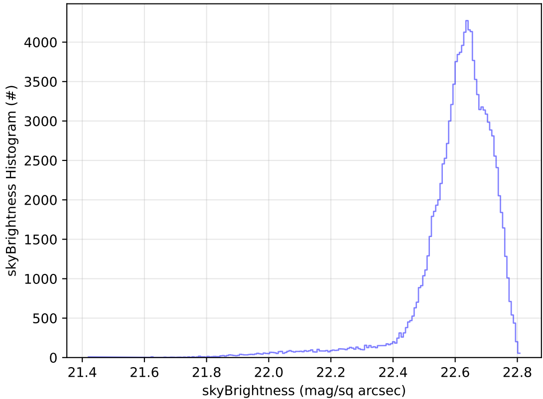
ddf_acor_sf10_lsf20_lsr10_v3.4_10yrs All sky u band: skyBrightness Histogram
