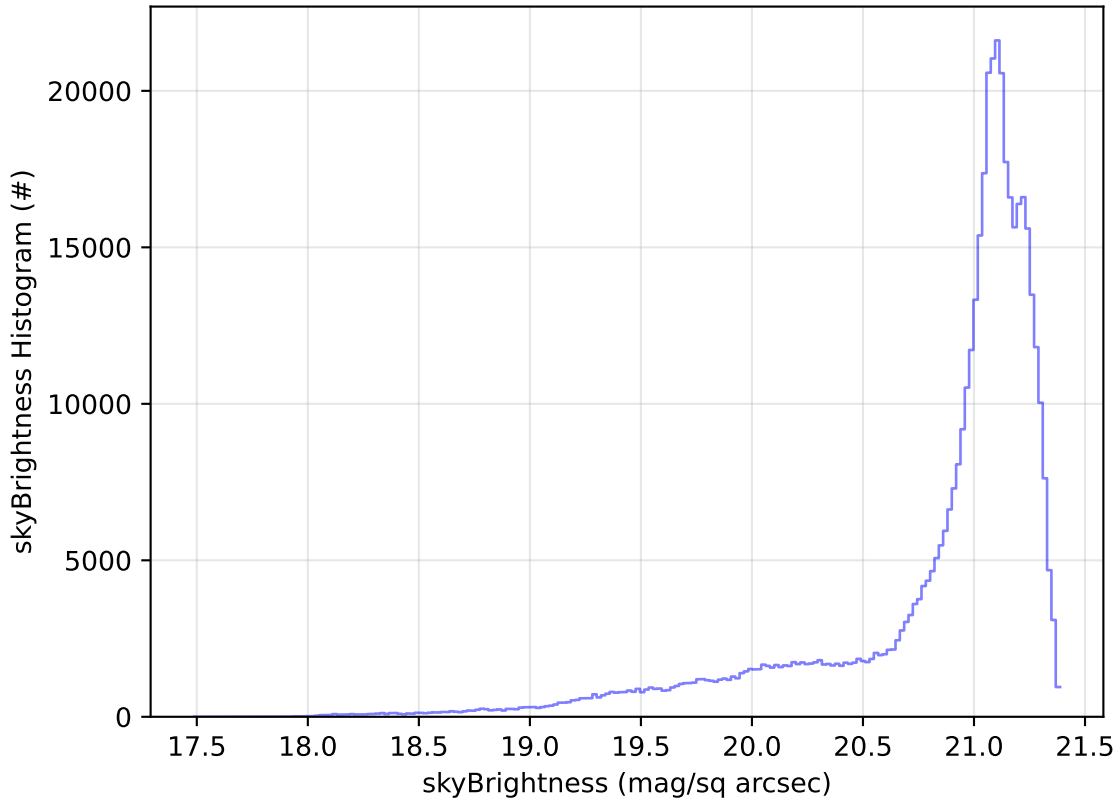
ddf_acor_sf10_lsf20_lsr10_v3.4_10yrs All sky r band: skyBrightness Histogram
