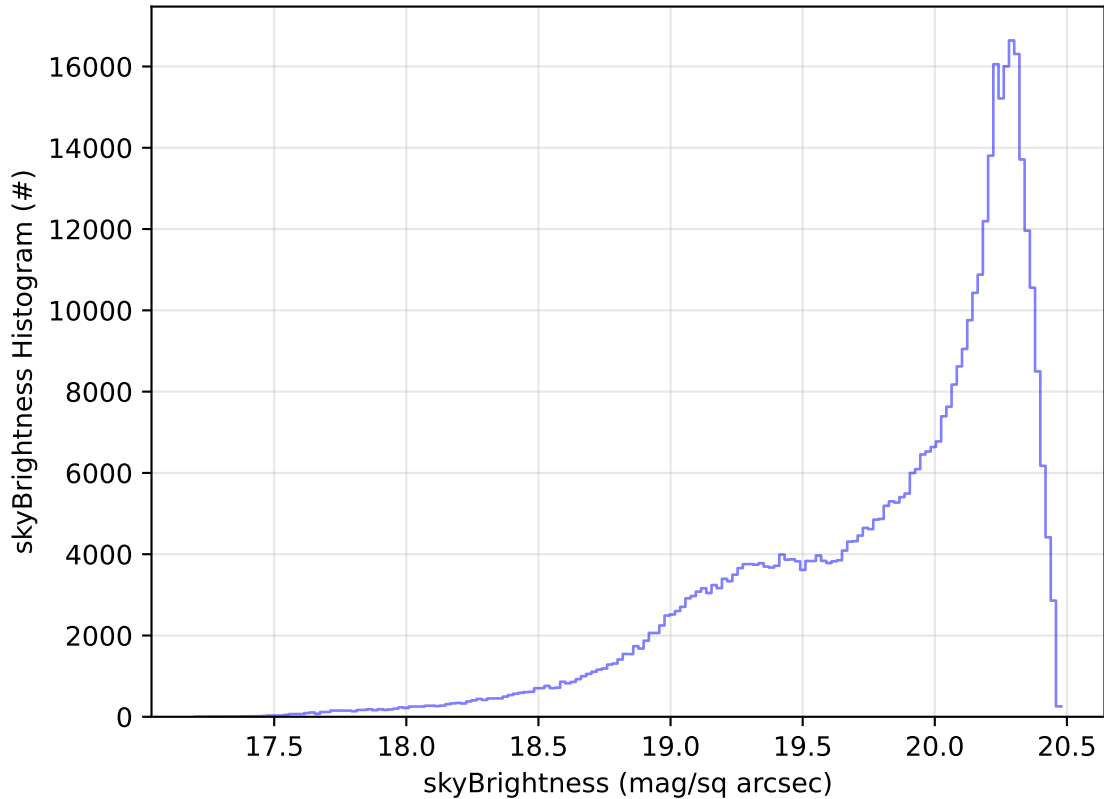
ddf_acor_sf10_lsf20_lsr10_v3.4_10yrs All sky i band: skyBrightness Histogram
