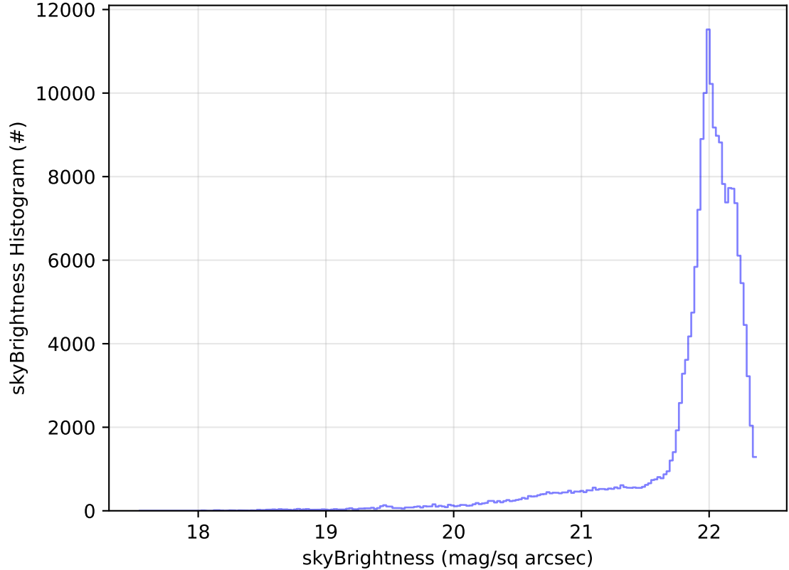
ddf_acor_sf10_lsf20_lsr10_v3.4_10yrs All sky g band: skyBrightness Histogram
