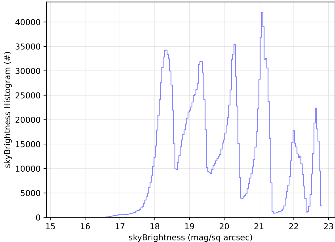
ddf_acor_sf10_lsf20_lsr10_v3.4_10yrs All sky all bands: skyBrightness Histogram
