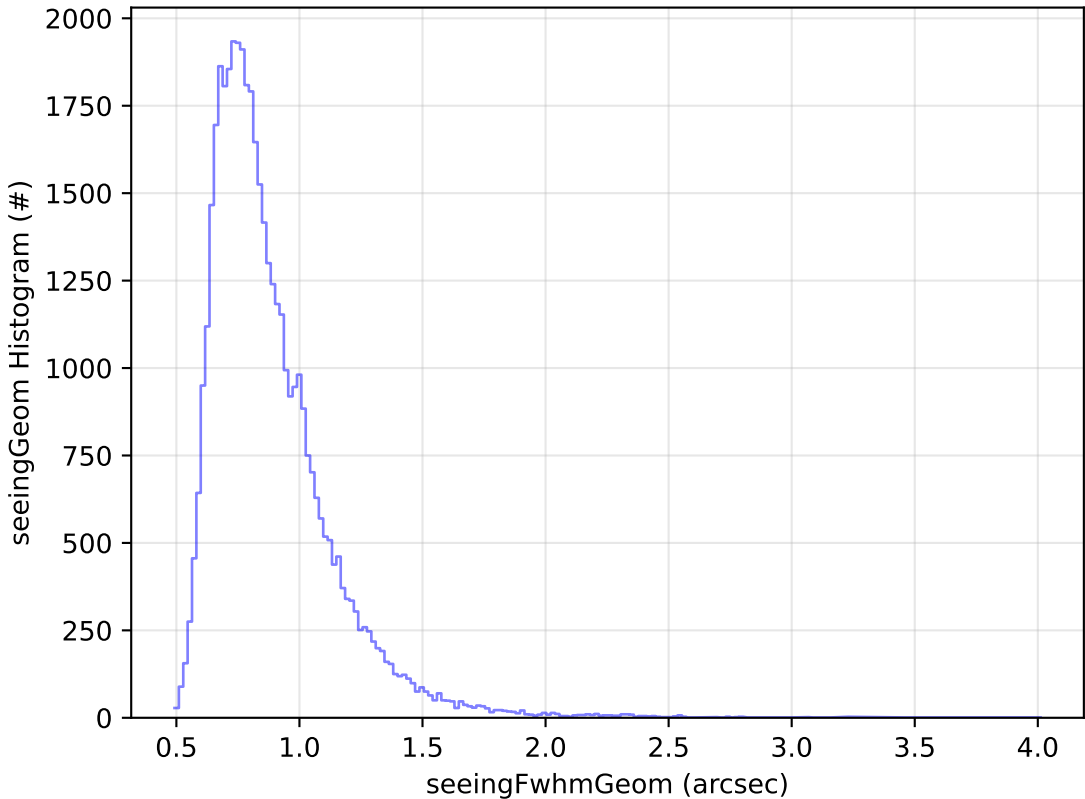
ddf_acor_sf10_lsf20_lsr10_v3.4_10yrs Yr 1 z band: seeingGeom Histogram
