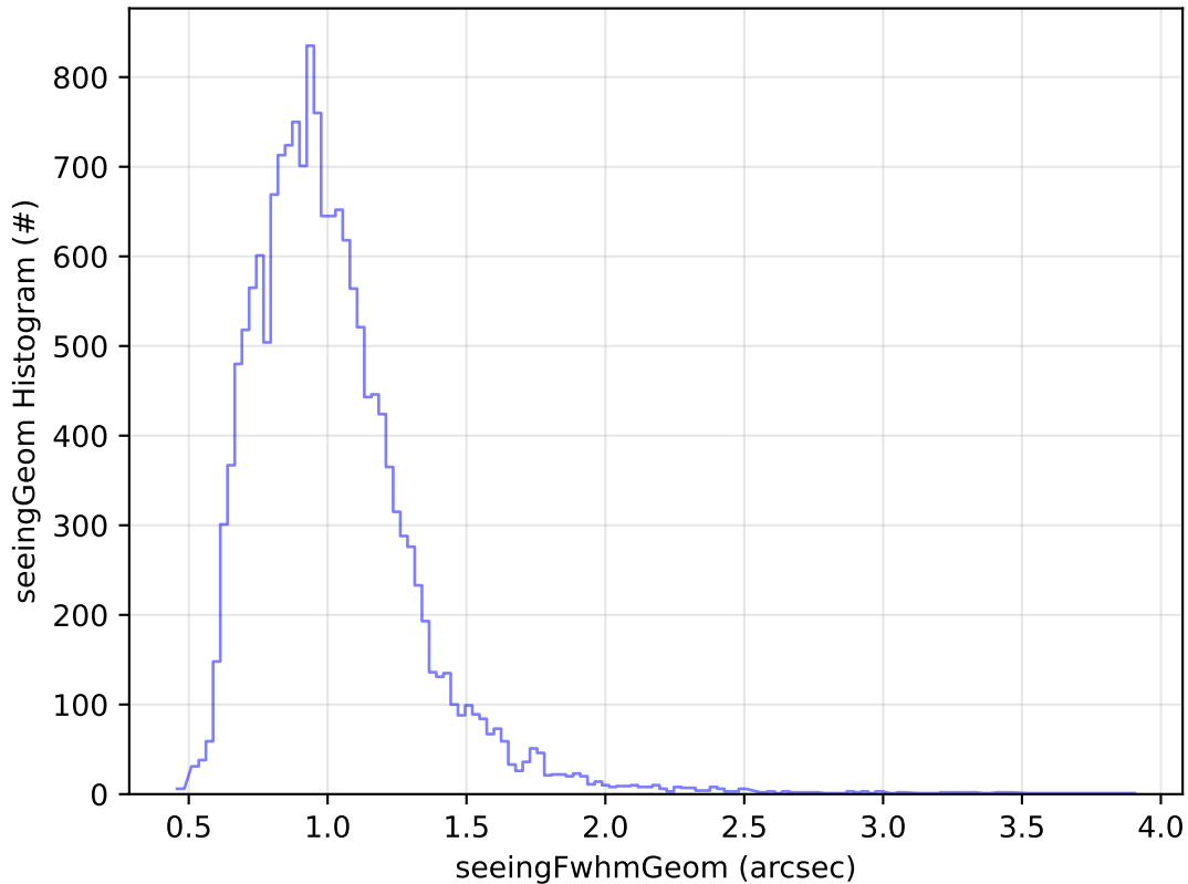
ddf_acor_sf10_lsf20_lsr10_v3.4_10yrs Yr 1 u band: seeingGeom Histogram
