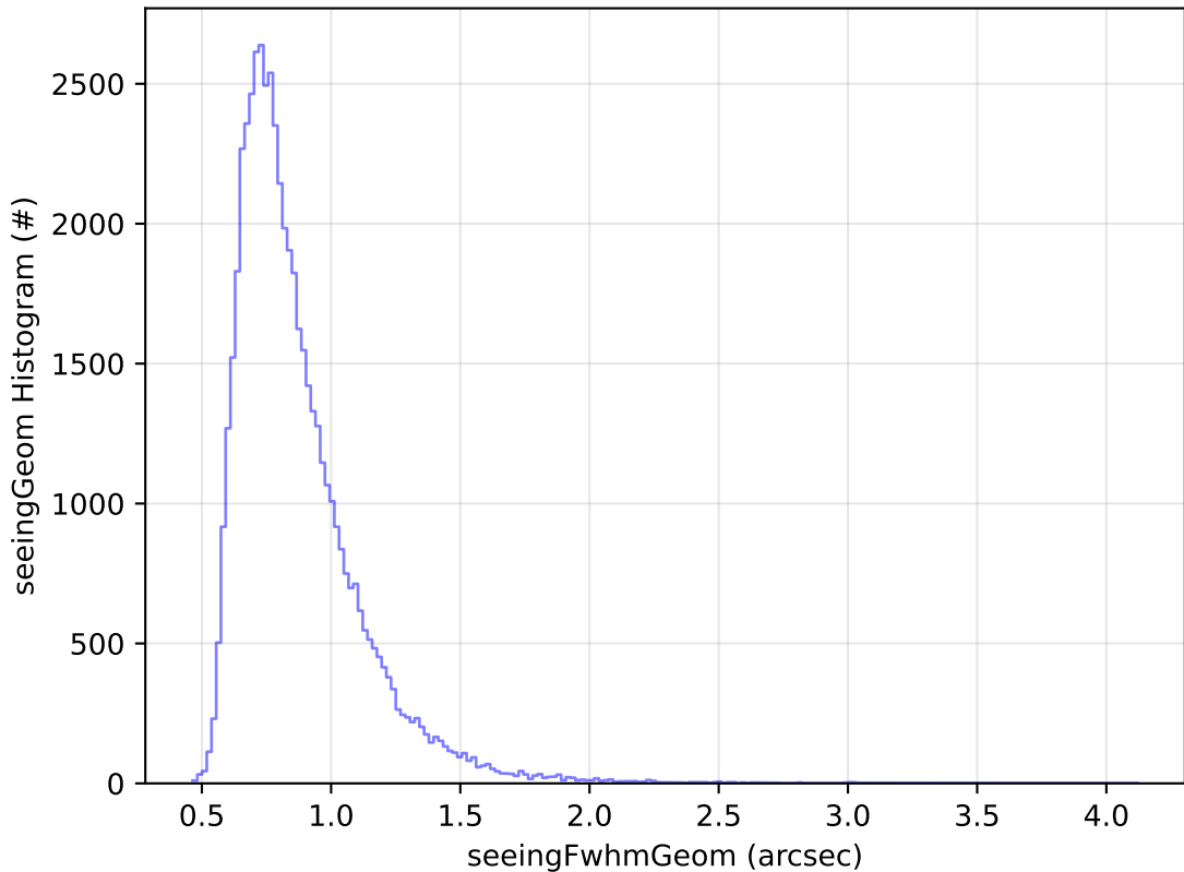
ddf_acor_sf10_lsf20_lsr10_v3.4_10yrs Yr 1 i band: seeingGeom Histogram
