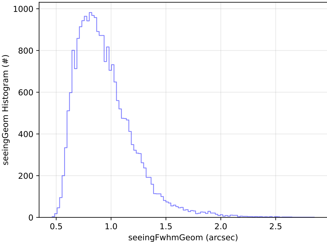
ddf_acor_sf10_lsf20_lsr10_v3.4_10yrs Yr 1 g band: seeingGeom Histogram
