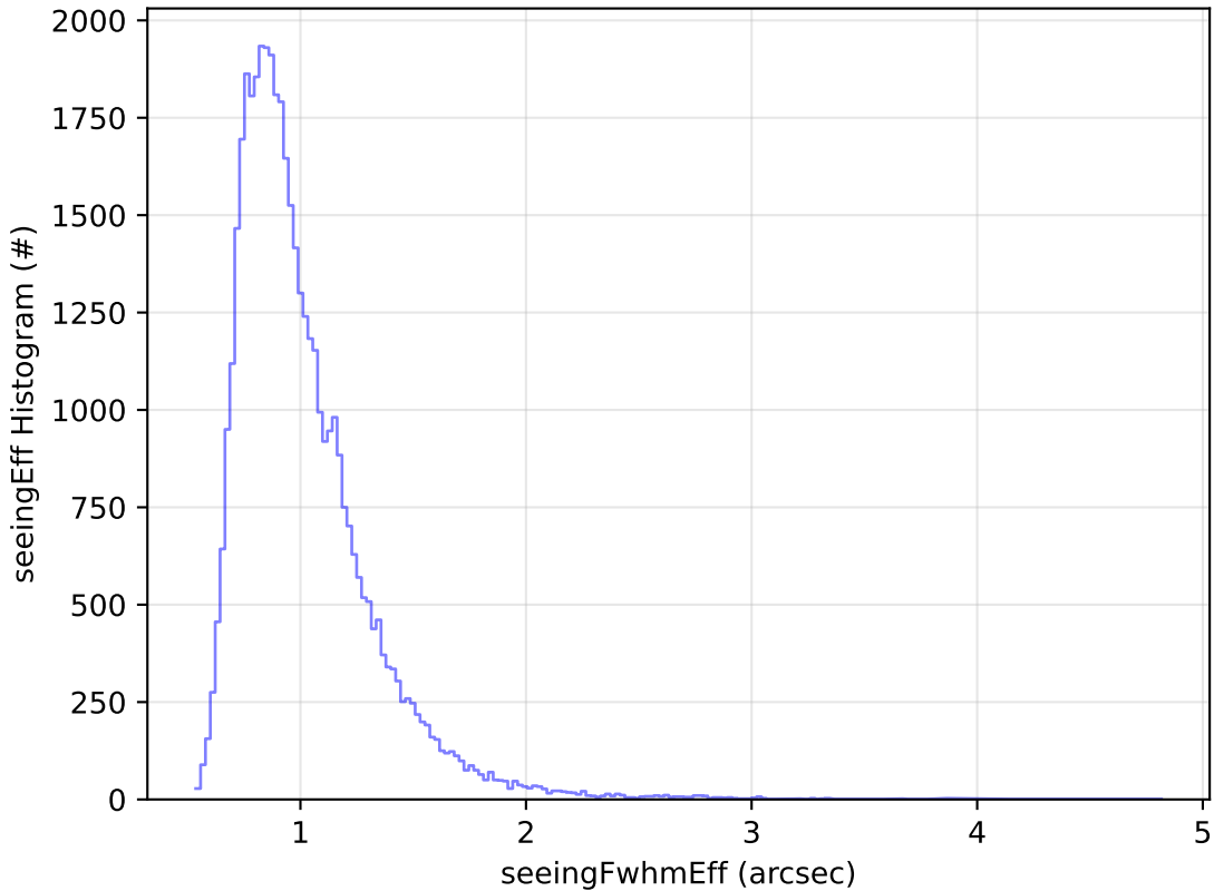
ddf_acor_sf10_lsf20_lsr10_v3.4_10yrs Yr 1 z band: seeingEff Histogram
