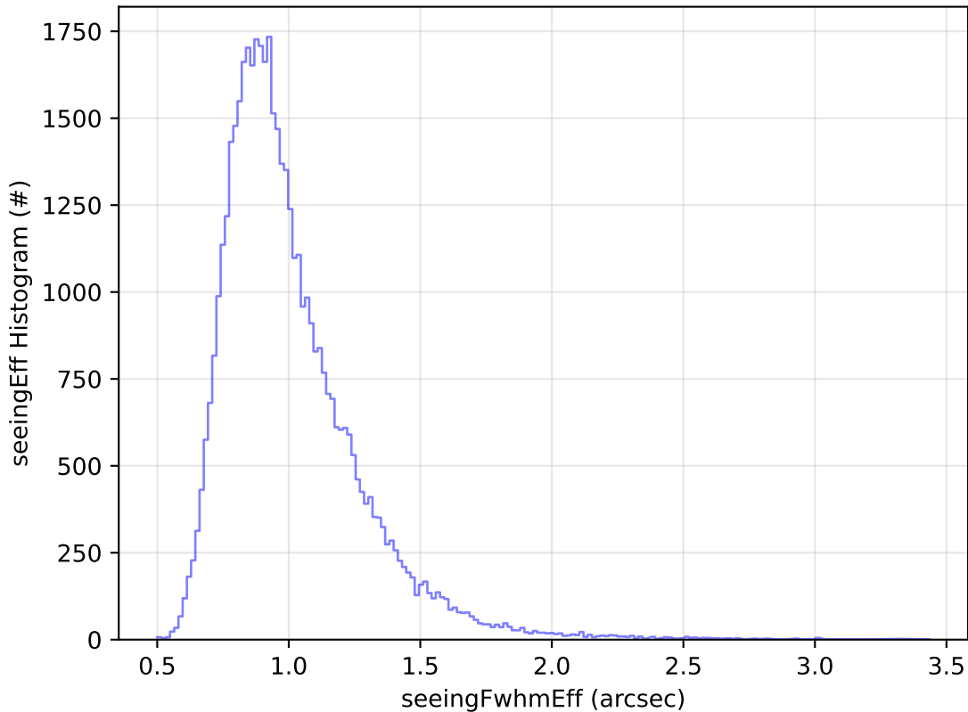
ddf_acor_sf10_lsf20_lsr10_v3.4_10yrs Yr 1 y band: seeingEff Histogram
