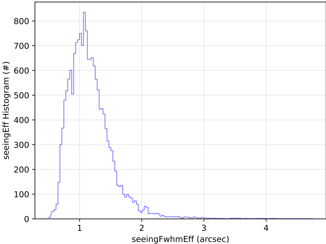
ddf_acor_sf10_lsf20_lsr10_v3.4_10yrs Yr 1 u band: seeingEff Histogram
