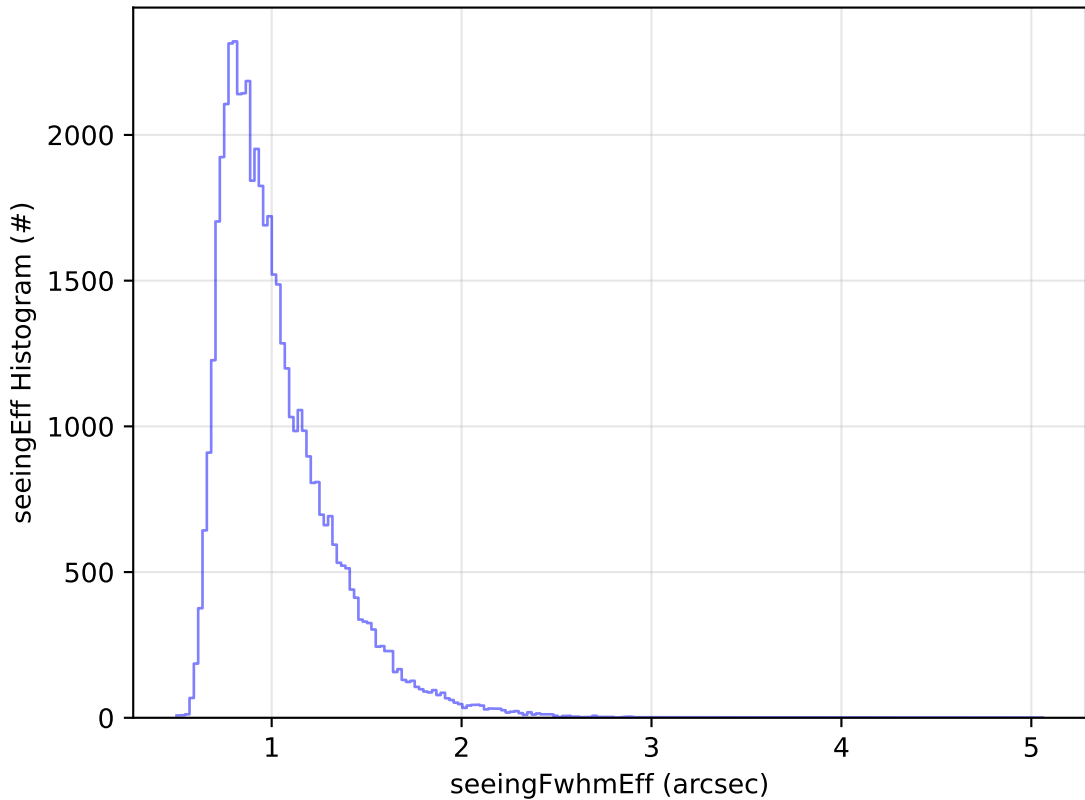
ddf_acor_sf10_lsf20_lsr10_v3.4_10yrs Yr 1 r band: seeingEff Histogram
