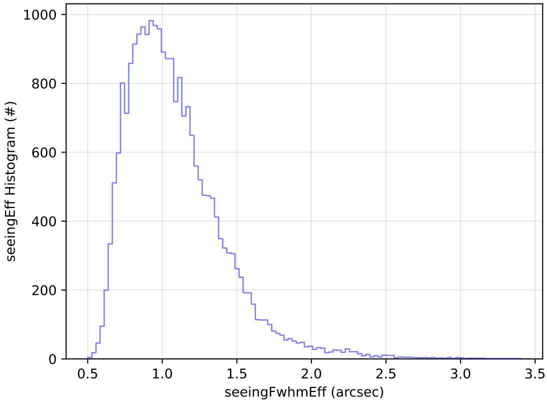
ddf_acor_sf10_lsf20_lsr10_v3.4_10yrs Yr 1 g band: seeingEff Histogram
