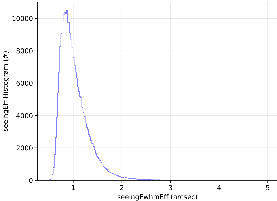
ddf_acor_sf10_Isf20_Isr10_v3.4_10yrs Yr 1 all bands: seeingEff Histogram
