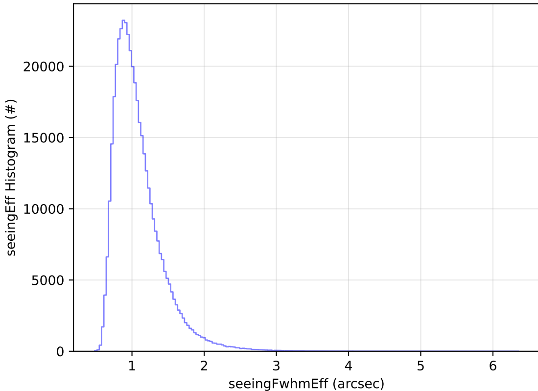
ddf_acor_sf10_lsf20_lsr10_v3.4_10yrs WFD z band: seeingEff Histogram
