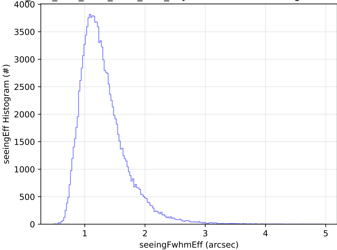
ddf_acor_sf10_lsf20_lsr10_v3.4_10yrs WFD u band: seeingEff Histogram
