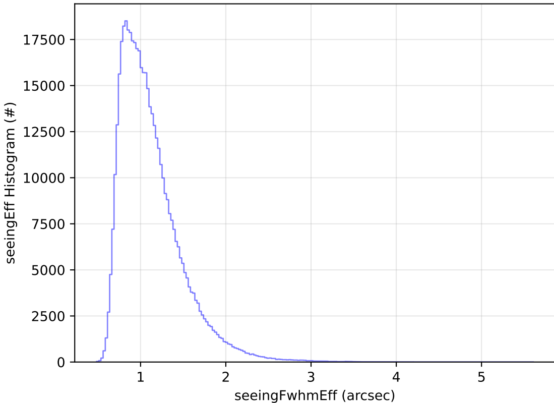
ddf_acor_sf10_lsf20_lsr10_v3.4_10yrs WFD r band: seeingEff Histogram
