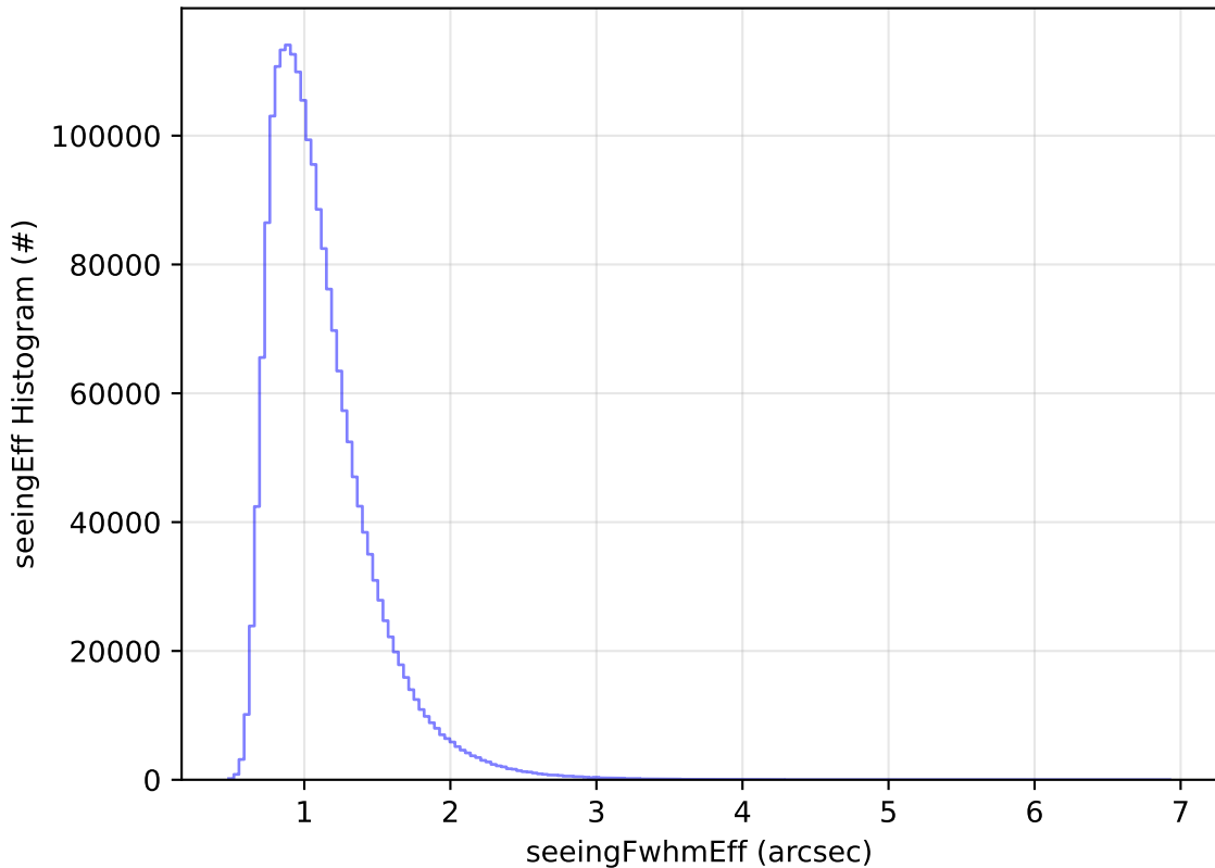
ddf_acor_sf10_lsf20_lsr10_v3.4_10yrs WFD all bands: seeingEff Histogram
