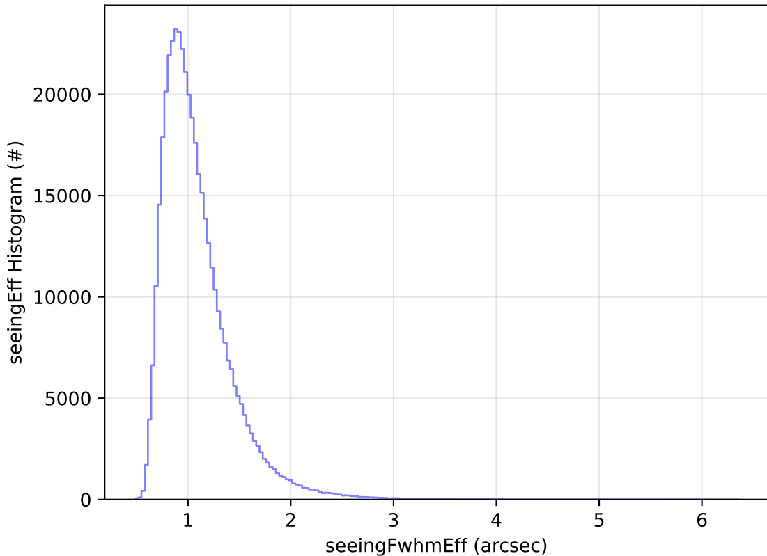
ddf_acor_sf10_lsf20_lsr10_v3.4_10yrs All sky z band: seeingEff Histogram
