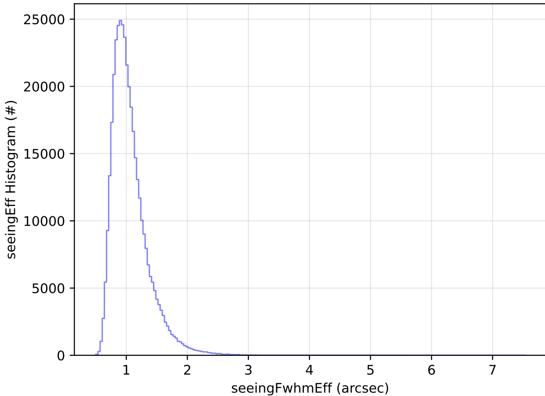
ddf_acor_sf10_lsf20_lsr10_v3.4_10yrs All sky y band: seeingEff Histogram
