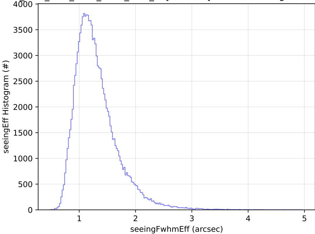
ddf_acor_sf10_ls20_lsr10_v3.4_10yrs All sky u band: seeingEff Histogram
