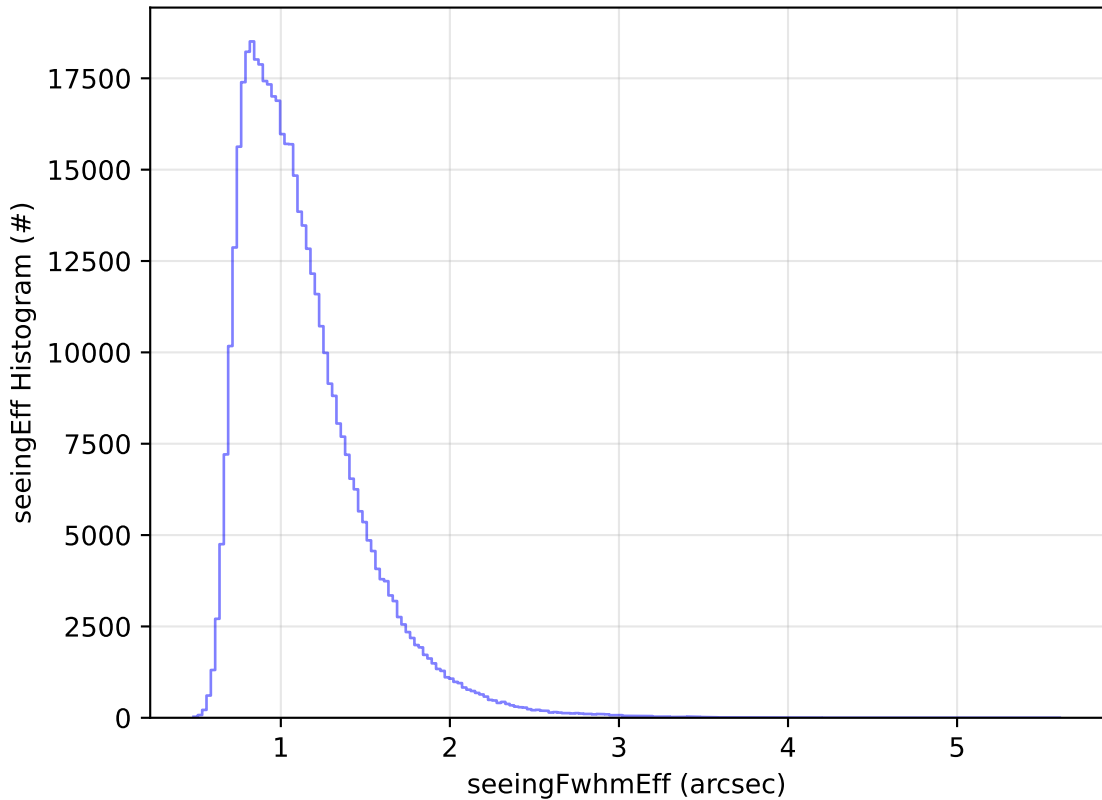
ddf_acor_sf10_lsf20_lsr10_v3.4_10yrs All sky r band: seeingEff Histogram
