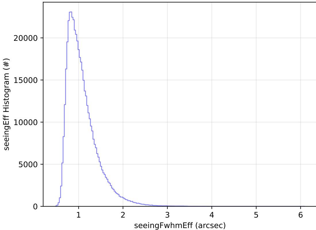
ddf_acor_sf10_lsf20_lsr10_v3.4_10yrs All sky i band: seeingEff Histogram
