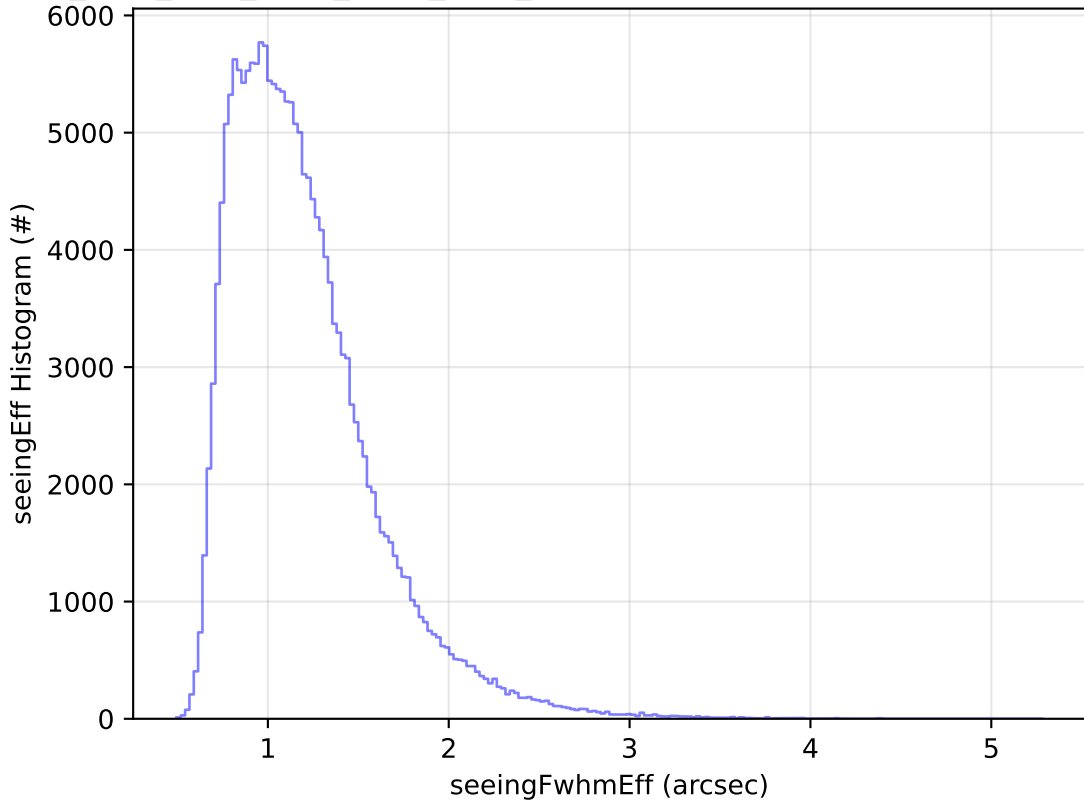
ddf_acor_sf10_ls20_lsr10_v3.4_10yrs All sky g band: seeingEff Histogram
