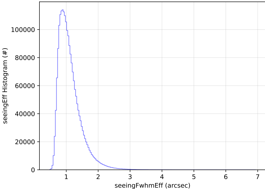
ddf_acor_sf10_lsf20_lsr10_v3.4_10yrs All sky all bands: seeingEff Histogram
