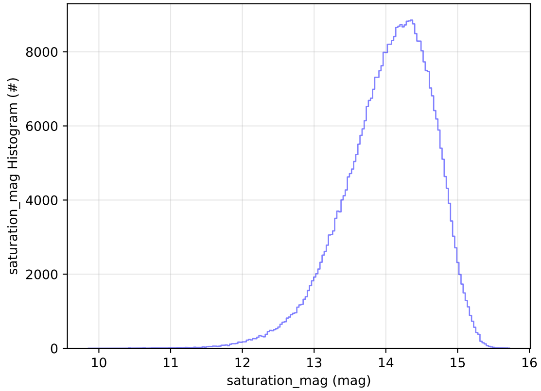
ddf_acor_sf10_lsf20_lsr10_v3.4_10yrs WFD z band: saturation_mag Histogram
