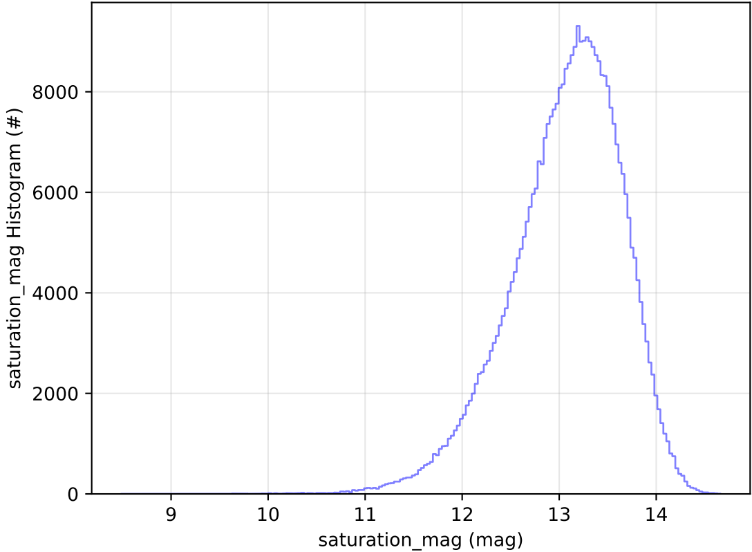
ddf_acor_sf10_lsf20_lsr10_v3.4_10yrs WFD y band: saturation_mag Histogram
