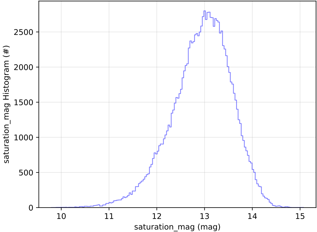
ddf_acor_sf10_lsf20_lsr10_v3.4_10yrs WFD u band: saturation_mag Histogram
