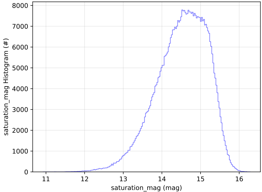
ddf_acor_sf10_lsf20_lsr10_v3.4_10yrs WFD r band: saturation_mag Histogram
