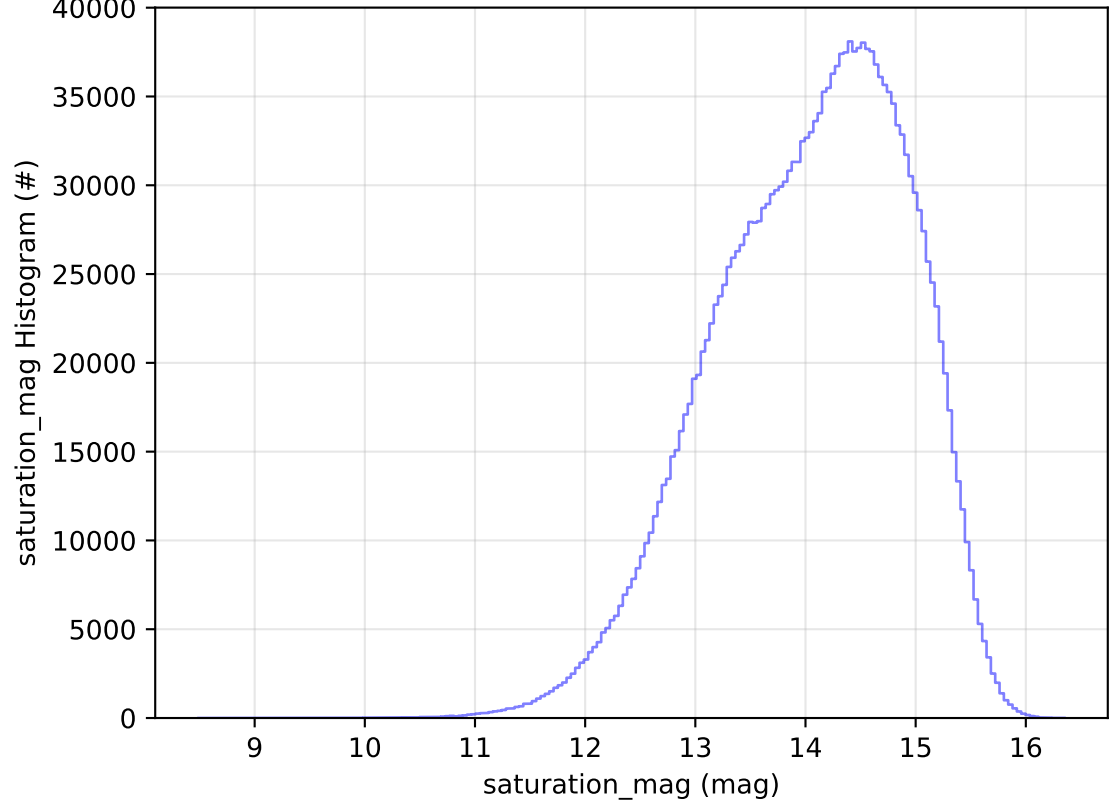
ddf_acor_sf10_lsf20_lsr10_v3.4_10yrs WFD all bands: saturation_mag Histogram
