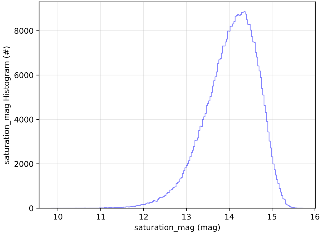
ddf_acor_sf10_lsf20_lsr10_v3.4_10yrs All sky z band: saturation_mag Histogram
