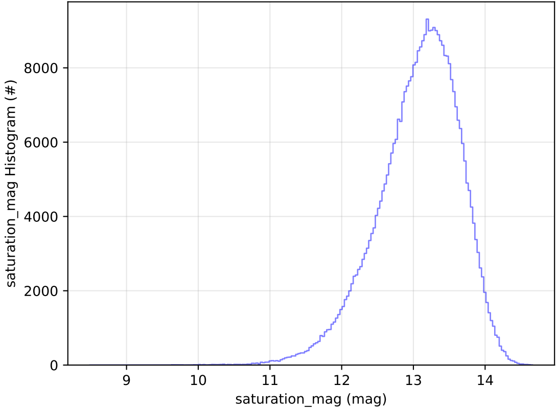
ddf_acor_sf10_lsf20_lsr10_v3.4_10yrs All sky y band: saturation_mag Histogram
