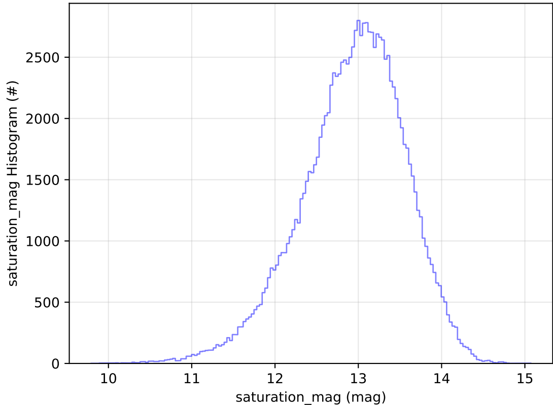
ddf_acor_sf10_lsf20_lsr10_v3.4_10yrs All sky u band: saturation_mag Histogram
