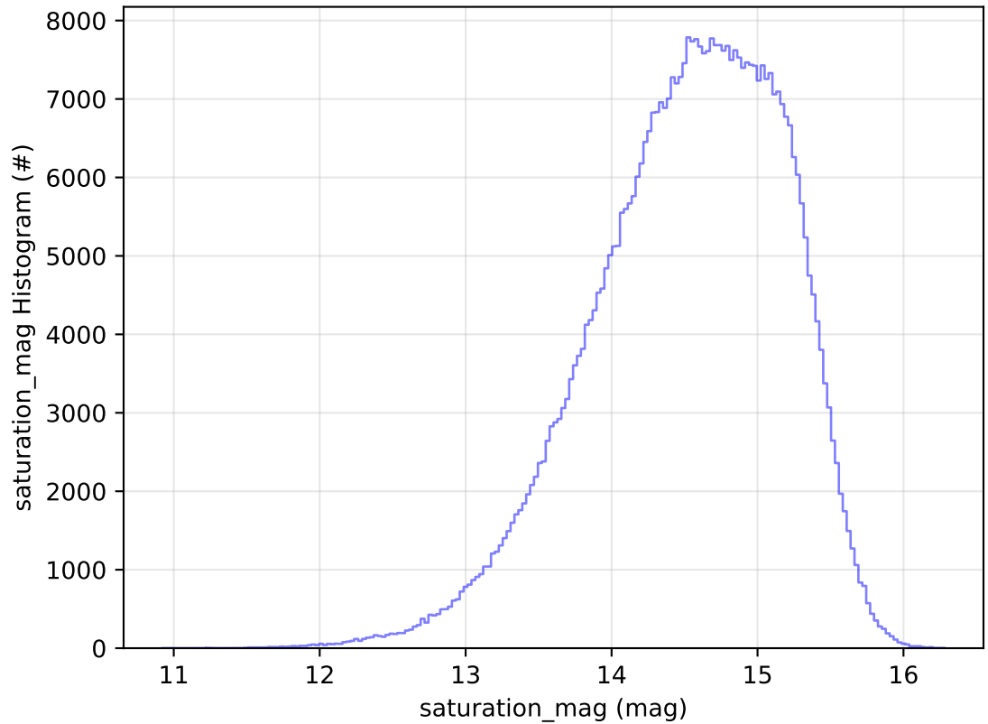
ddf_acor_sf10_lsf20_lsr10_v3.4_10yrs All sky r band: saturation_mag Histogram
