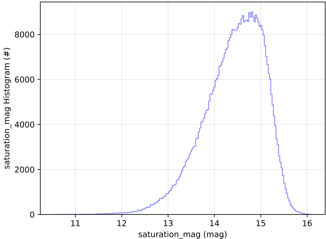
ddf_acor_sf10_lsf20_lsr10_v3.4_10yrs All sky i band: saturation_mag Histogram
