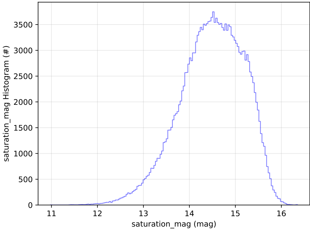
ddf_acor_sf10_lsf20_lsr10_v3.4_10yrs All sky g band: saturation_mag Histogram
