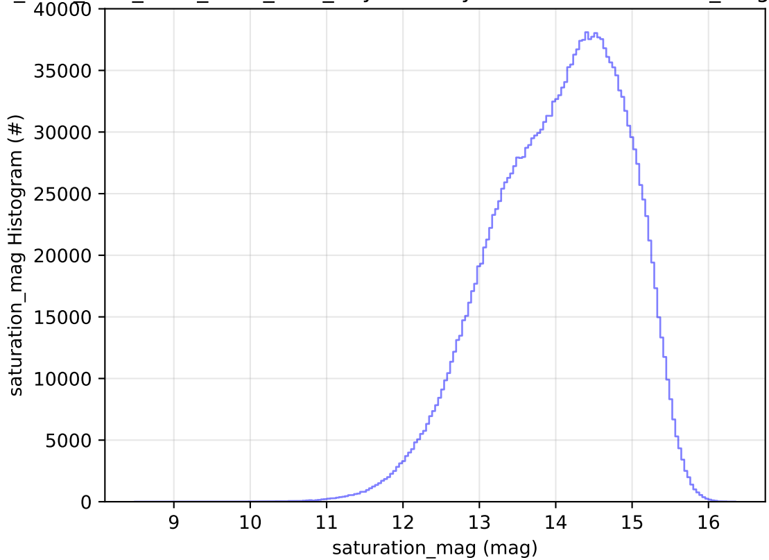
ddf_acor_sf10_lsf20_lsr10_v3.4_10yrs All sky all bands: saturation_mag Histogram
