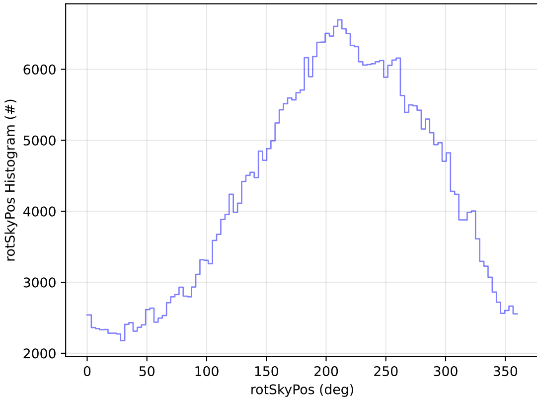
ddf_acor_sf10_lsf20_lsr10_v3.4_10yrs WFD z band: rotSkyPos Histogram
