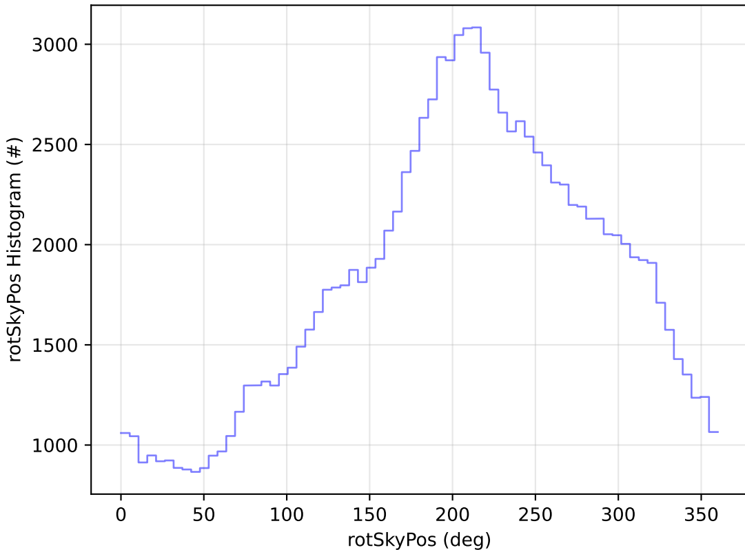
ddf_acor_sf10_lsf20_lsr10_v3.4_10yrs WFD u band: rotSkyPos Histogram
