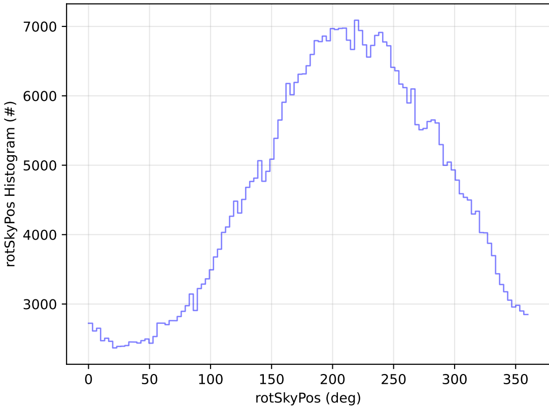
ddf_acor_sf10_lsf20_lsr10_v3.4_10yrs WFD i band: rotSkyPos Histogram
