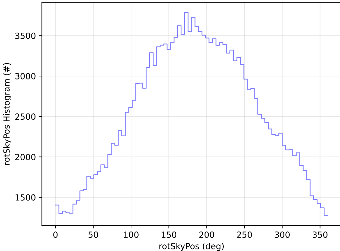
ddf_acor_sf10_lsf20_lsr10_v3.4_10yrs WFD g band: rotSkyPos Histogram
