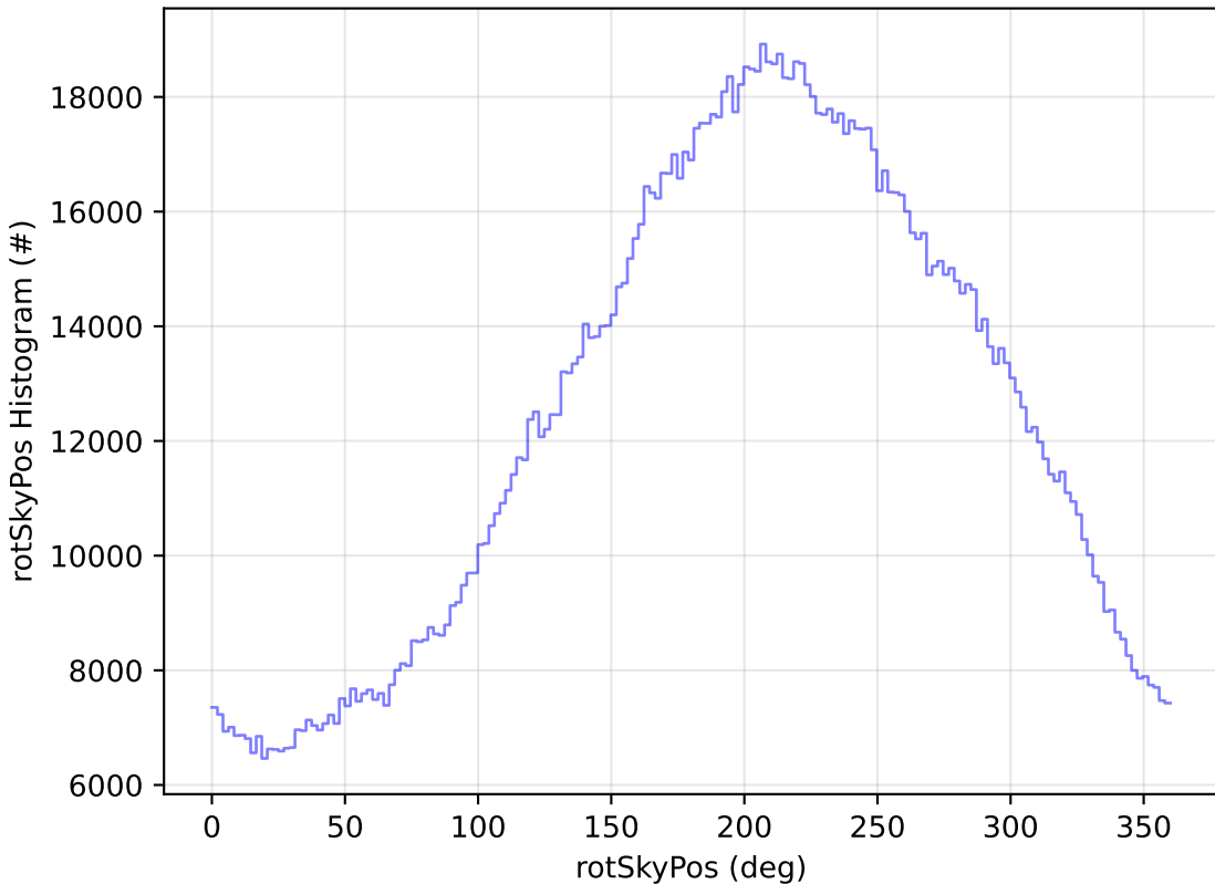
ddf_acor_sf10_lsf20_lsr10_v3.4_10yrs WFD all bands: rotSkyPos Histogram
