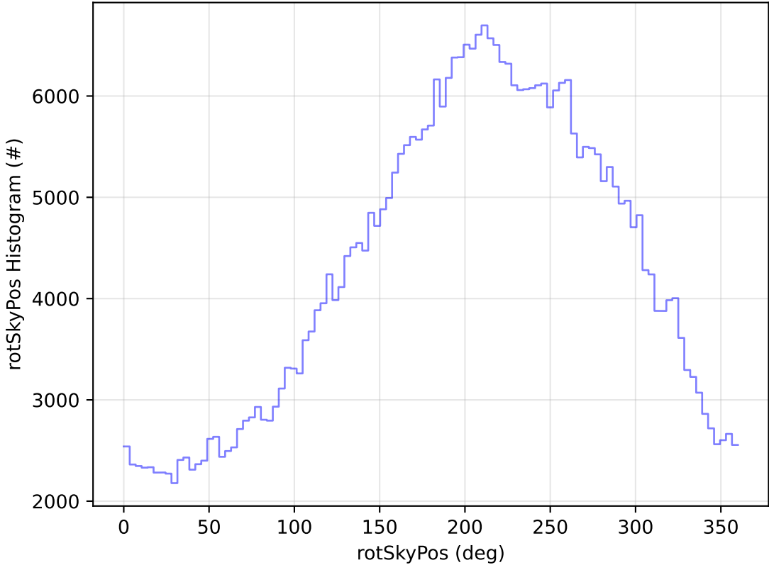
ddf_acor_sf10_lsf20_lsr10_v3.4_10yrs All sky z band: rotSkyPos Histogram
