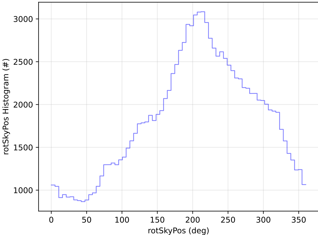
ddf_acor_sf10_lsf20_lsr10_v3.4_10yrs All sky u band: rotSkyPos Histogram
