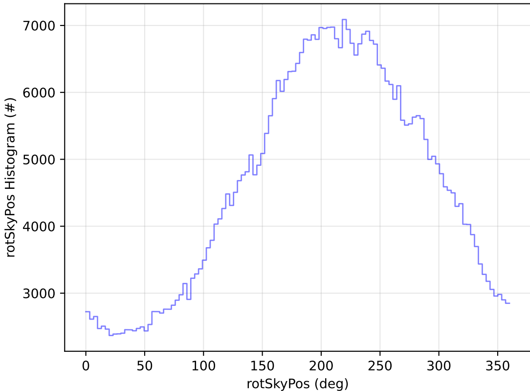
ddf_acor_sf10_lsf20_lsr10_v3.4_10yrs All sky i band: rotSkyPos Histogram
